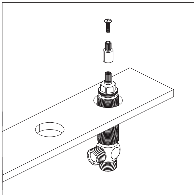
Insert extension and screw onto the valve
