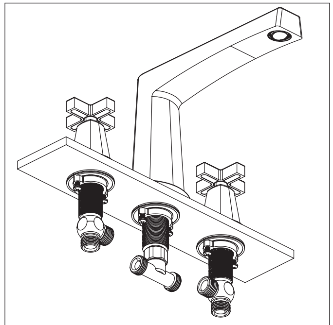
Remove T-fitting
