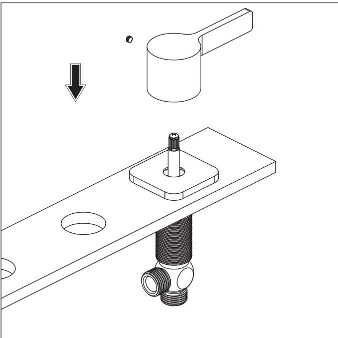
Install handle from top of deck and tighten hex screw
