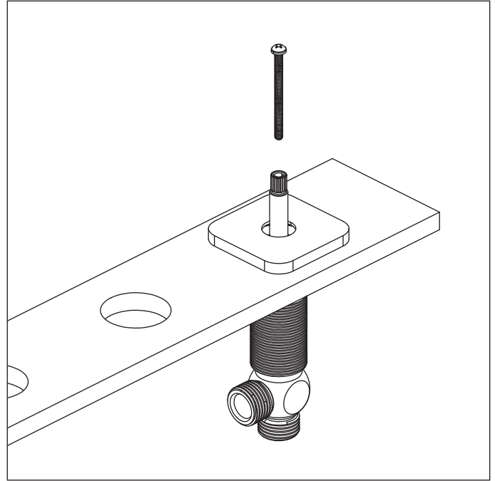
Install screw from top of deck and tighten
