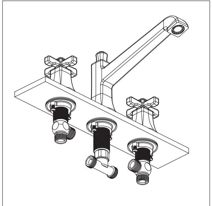
Remove T-fitting
