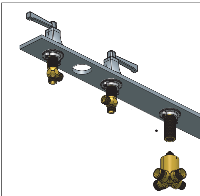
Install the diverter body from bottom
