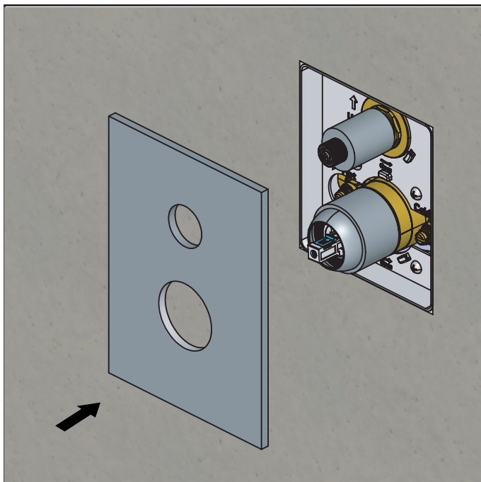
Fix the trim on wall apply silicon behind the trim plate
