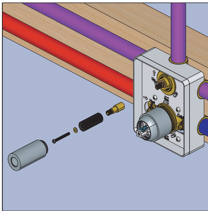
Insert Diverter extension
