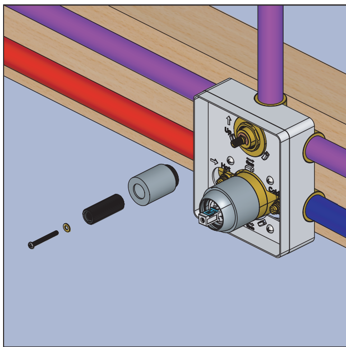
Remove diverter trim piece
