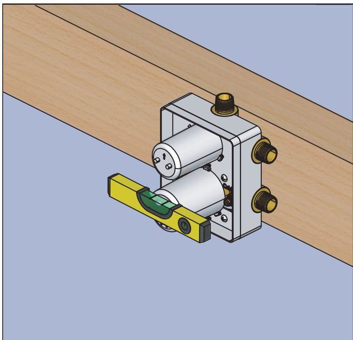
Level Valve
