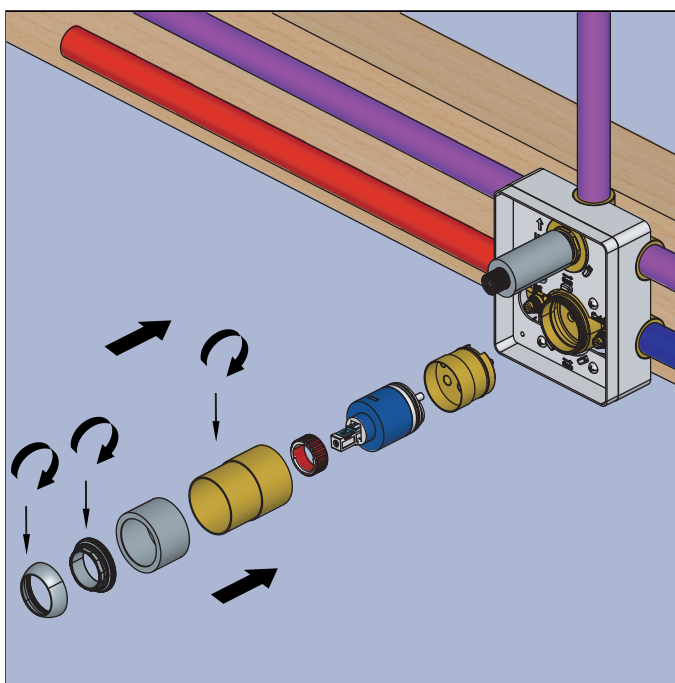
Insert temperature extension piece, extended cartridge cover, Temperature cartridge, retaining nut and bezel.
