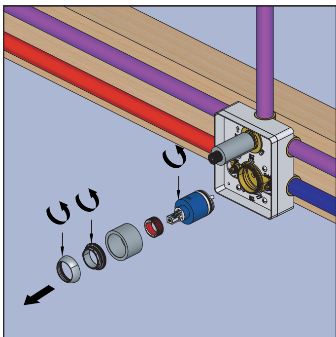
Remove temperature cartridge and cartridge cover
