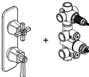
Trim [270.4000VT**]
